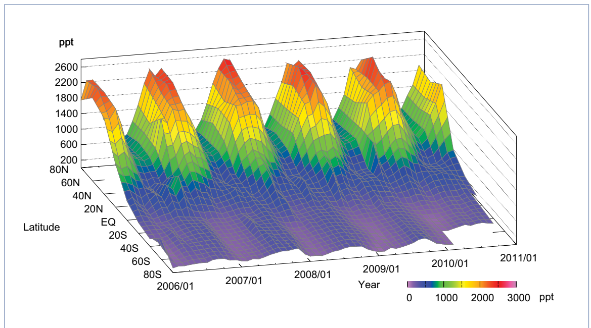
Figure 12. Monthly mean latitudinal variation of ethane from the global reactive gases measurements in the GAW network (Source: World Data Centre for Greenhouse Gases)
